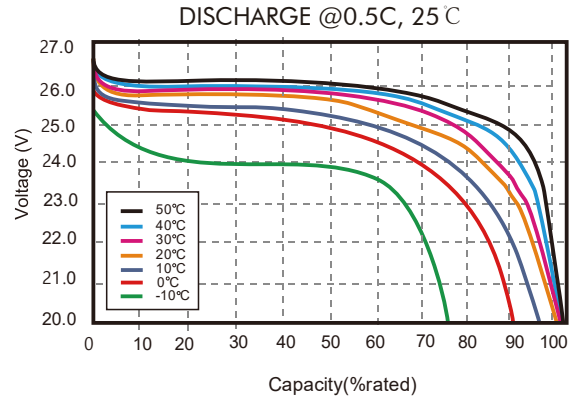
DISCHARGE CAPACITY at VARIOUS TEMPERATURES
